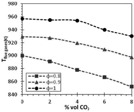
Figure 13. Temperatures of flue gases with O 2 enrichment (left) and CO 2 dilution (right) for Sn=0.8 at three equivalence ratios \phi=0.8 , 0.9 and 1.
