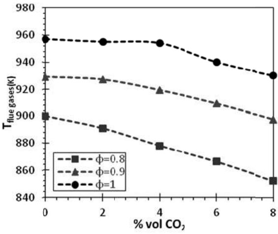
Figure 13. Temperatures of flue gases with \text{O}_2 enrichment (left) and \text{CO}_2 dilution (right) for \text{Sn}=0.8 at three equivalence ratios \phi=0.8, 0.9 and 1 .
