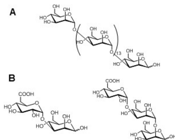
Figure 3. Drawings of hypothetical structures of oligosaccharides found in insoluble cell wall polysaccharides after mild acid hydrolysis of Phaeodactylum tricornutum cell wall extracts. (A) 1,3-linked mannopyranose chains; (B) oligosaccharide fragments. Although hypothetical alpha-linkages are shown here, there is no clear evidence for either alpha- or beta-linkages [65].
