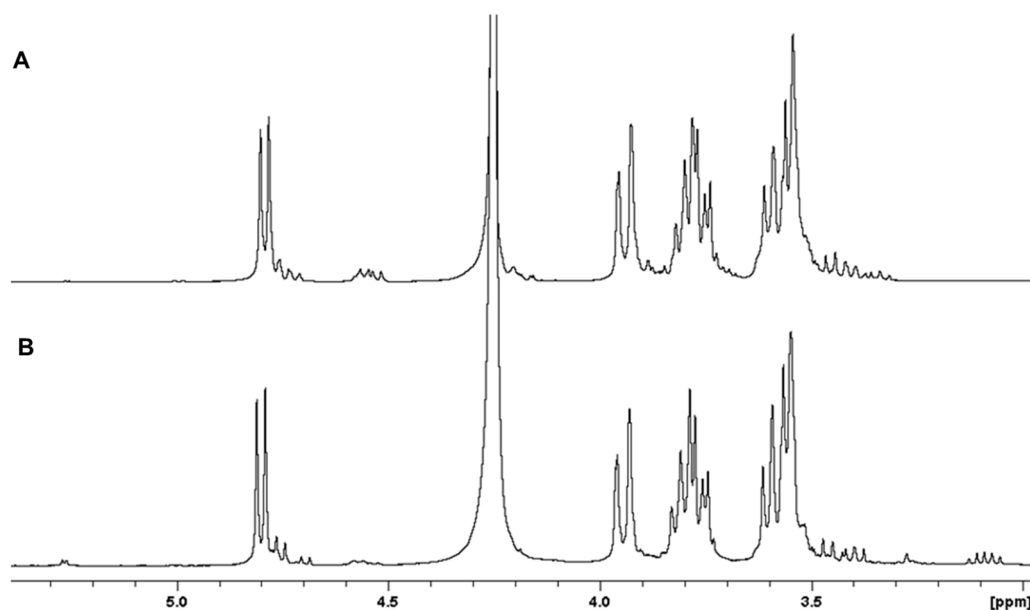
Figure 5. Structural analysis of \beta(1,3) glucan, a food storage polysaccharide. ^1\text{H} NMR spectra of (A) laminarin from Saccharina latissima and (B) \beta(1,3) glucan (chrysolaminarin) extracted from Phaeodactylum tricornutum (400 MHz, 353 K). Chrysolaminarin contains fewer \beta(1,6) branching signals (4.5–4.6 ppm) than laminarin. The slightly higher reducing end signal at 5.26 ppm ( \alpha -anomer) in the chrysolaminarin spectrum can be attributed to a lower molecular weight or the absence of a mannitol residue at the reducing end.
