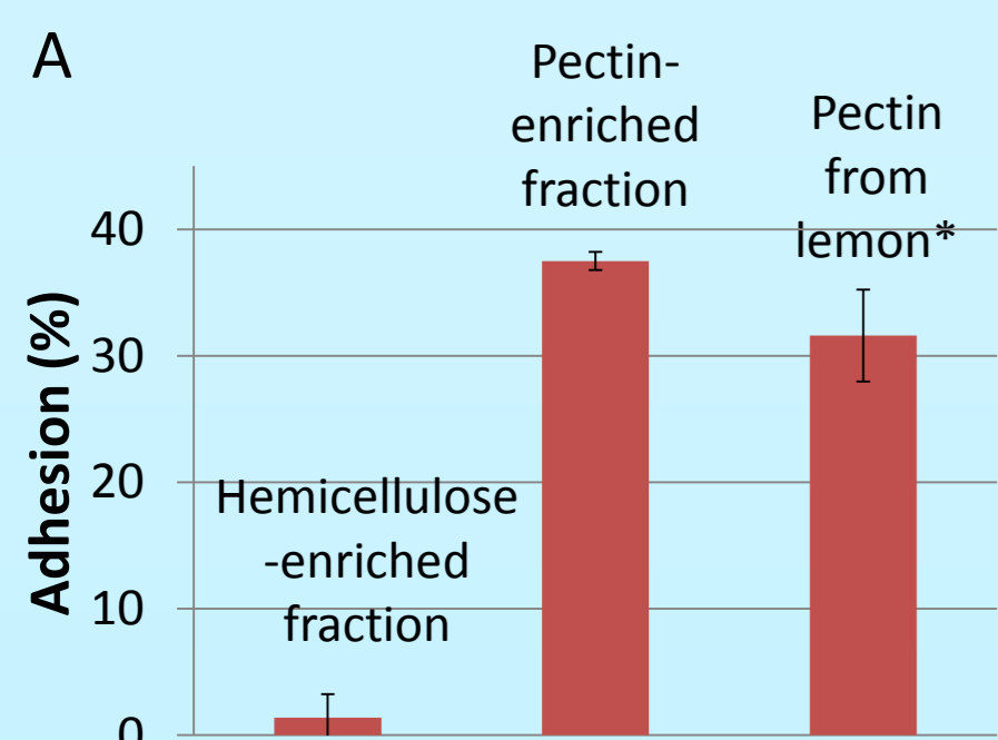
Figure 1: (A) Effect of pectin and hemicellulose-enriched fractions on pollen tube adhesion. (B) Monosaccharide composition by gas chromatography of the fractions. HG and RG-I backbone levels are indicated. * Pectin from lemon, 85 % degree of methylesterification (DM) (Sigma-Aldrich ® ).
