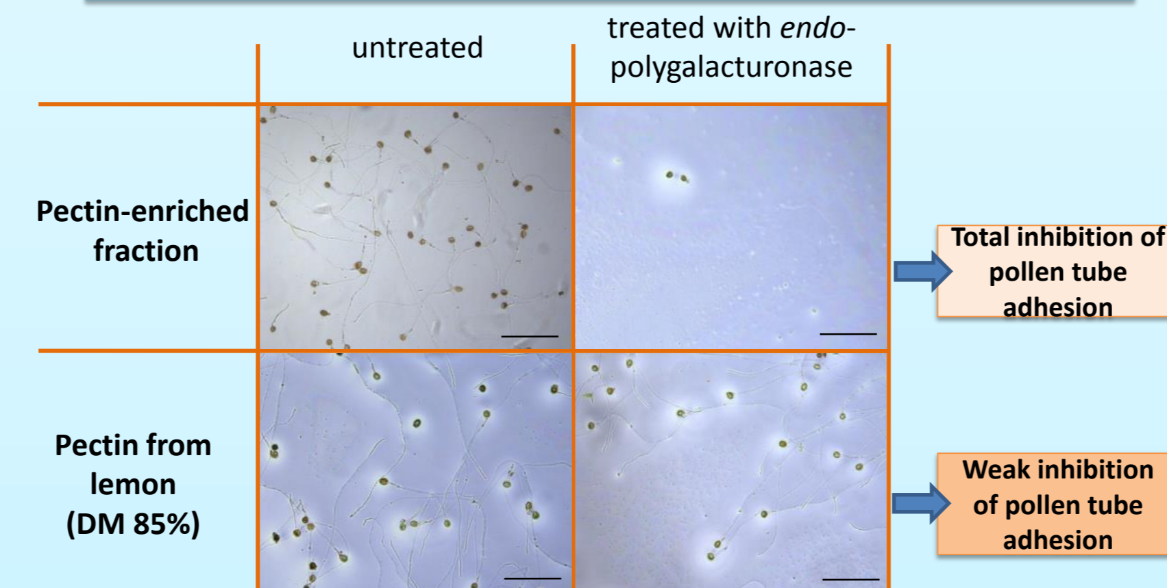
Figure 3: An endo -polygalacturonase treatment on the pectin-enriched fraction and on pectin from lemon (DM = 85%). Pictures show pollen tubes remaining on the matrix after the washing step. scale bar = 200 µm.
