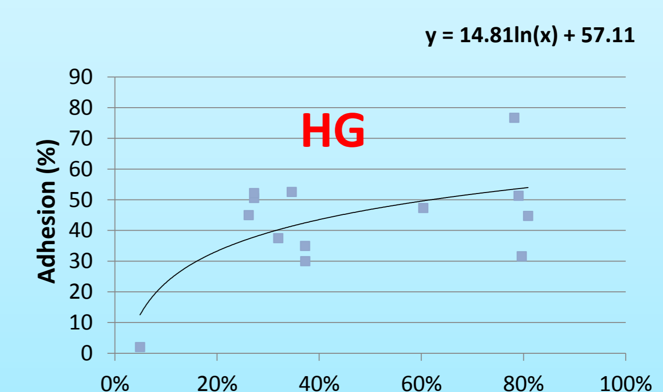
Figure 6: Effect of HG levels in pectin-enriched extracts on the adhesion rates.
