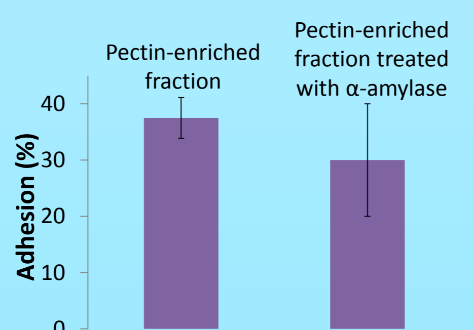
Figure 2: Effect of an \alpha -amylase treatment of the pectin-enriched fraction on pollen tube adhesion.
