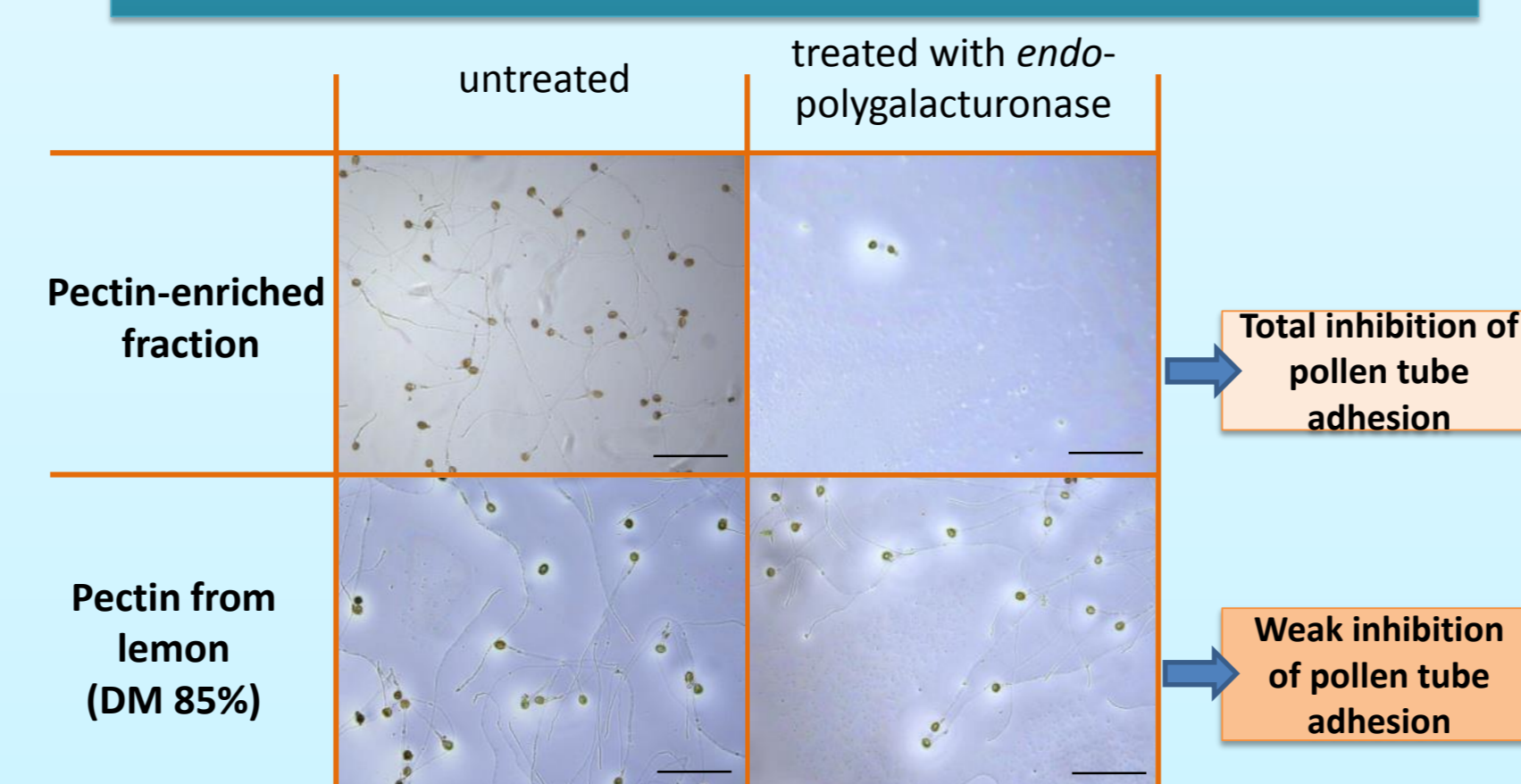
Figure 3: An endo -polygalacturonase treatment on the pectin-enriched fraction and on pectin from lemon (DM = 85%). Pictures show pollen tubes remaining on the matrix after the washing step. scale bar = 200 µm.
