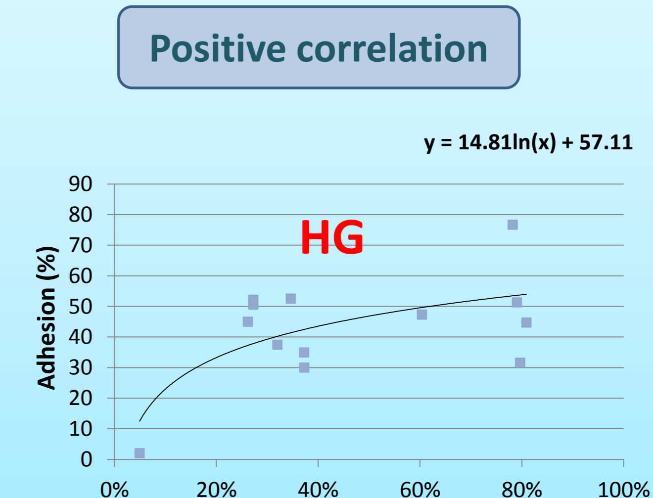
Figure 6: Effect of HG levels in pectin-enriched extracts on the adhesion rates.
