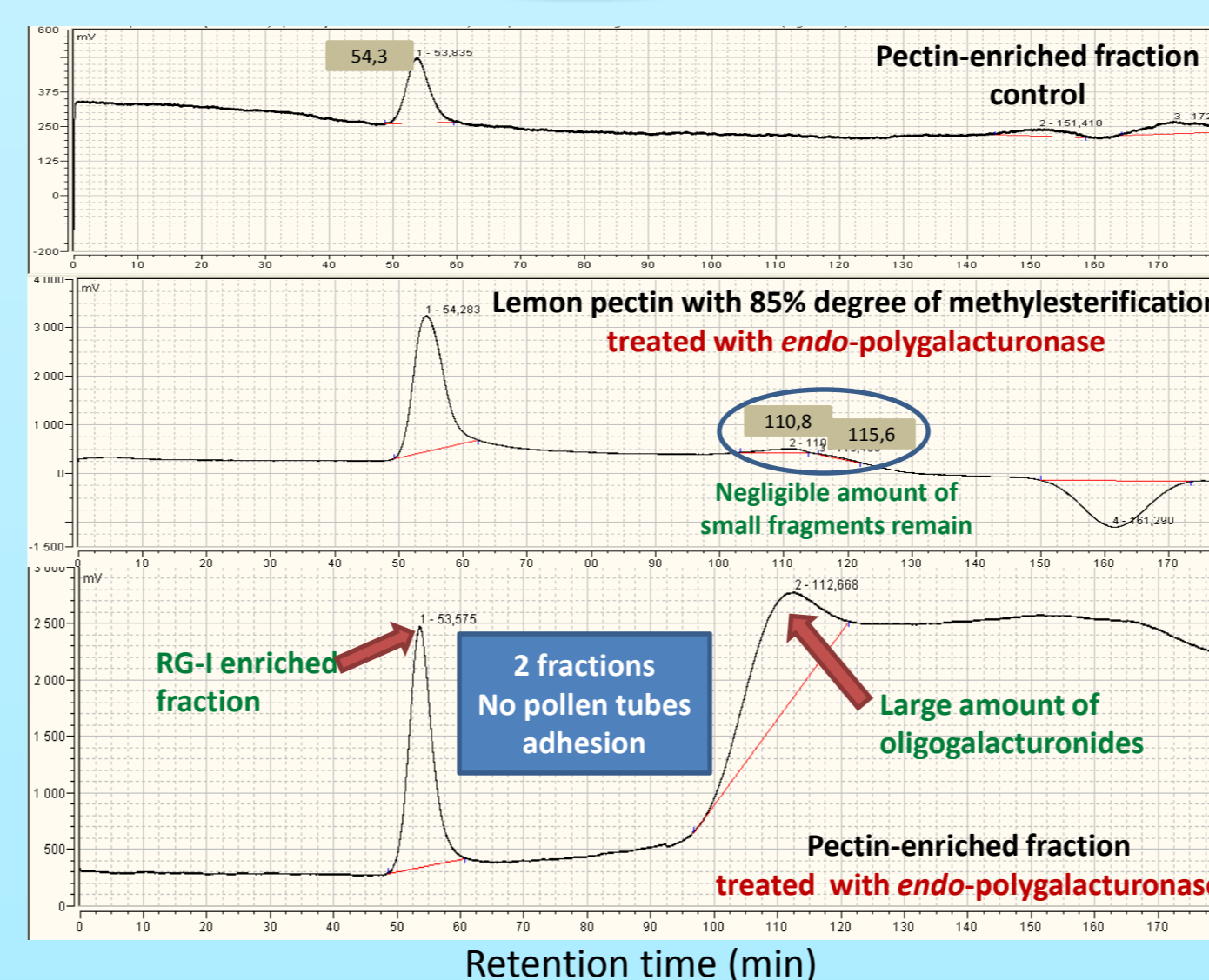
Figure 4: Size Exclusion Chromatography (SEC) performed on Sephadex-75G (fractionation range 3 \times 10^3 - 8 \times 10^4 Da) of untreated and treated pectin enriched-fraction and pectin from lemon with endo -polygalacturonase.
