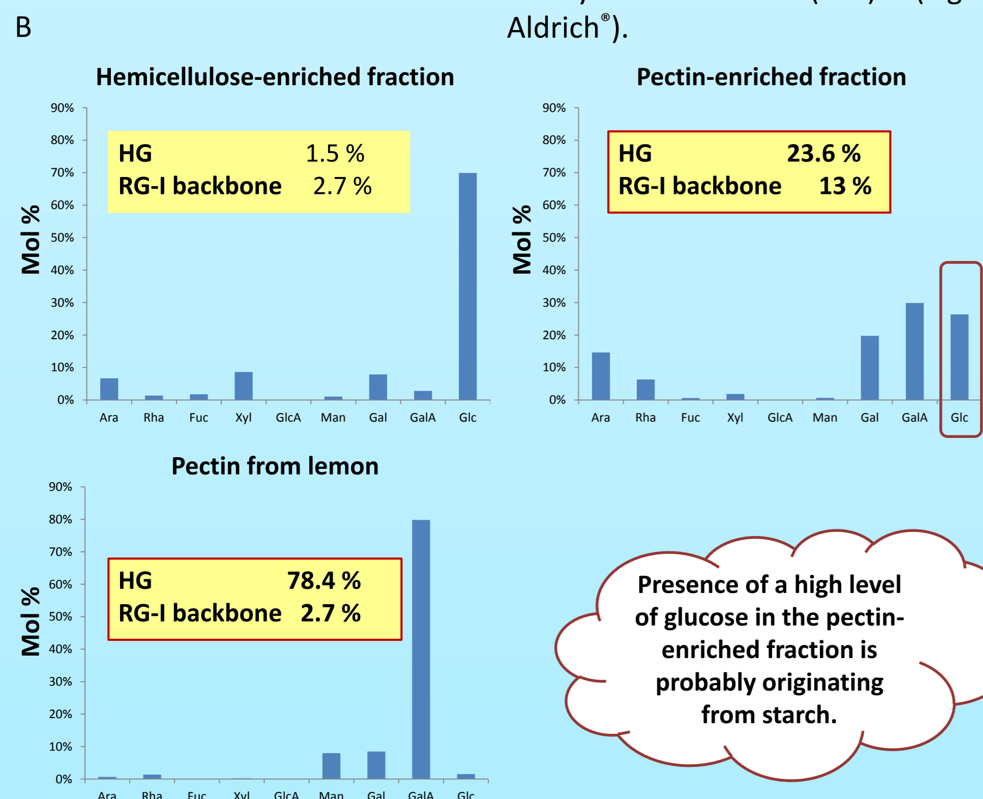
Figure 1: (A) Effect of pectin and hemicellulose-enriched fractions on pollen tube adhesion. (B) Monosaccharide composition by gas chromatography of the fractions. HG and RG-I backbone levels are indicated. * Pectin from lemon, 85 % degree of methylesterification (DM) (Sigma-Aldrich ® ).
