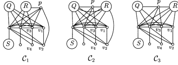
Figure 5: Examples of tree-perfect graphs [8]. The sets Q, R, S represent modules substituting the vertices q, r, v_n .
