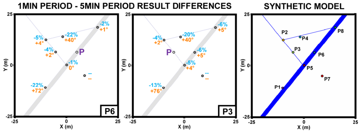
Figure 5: Differences in relative amplitude (in blue, in %) and relative phase offset (in orange, in ^{\circ} ) values in the oscillatory responses by decreasing from a 5 min period signal to a 1 min period signal for two different harmonic pumping locations (P6, P3). A dash represents an absence of oscillatory response (< 1 mm). The pumping location is indicated by 'P'. The main signal differences appear for the boreholes located in the matrix, near to a conduit (P1, P4) (dual connection).
