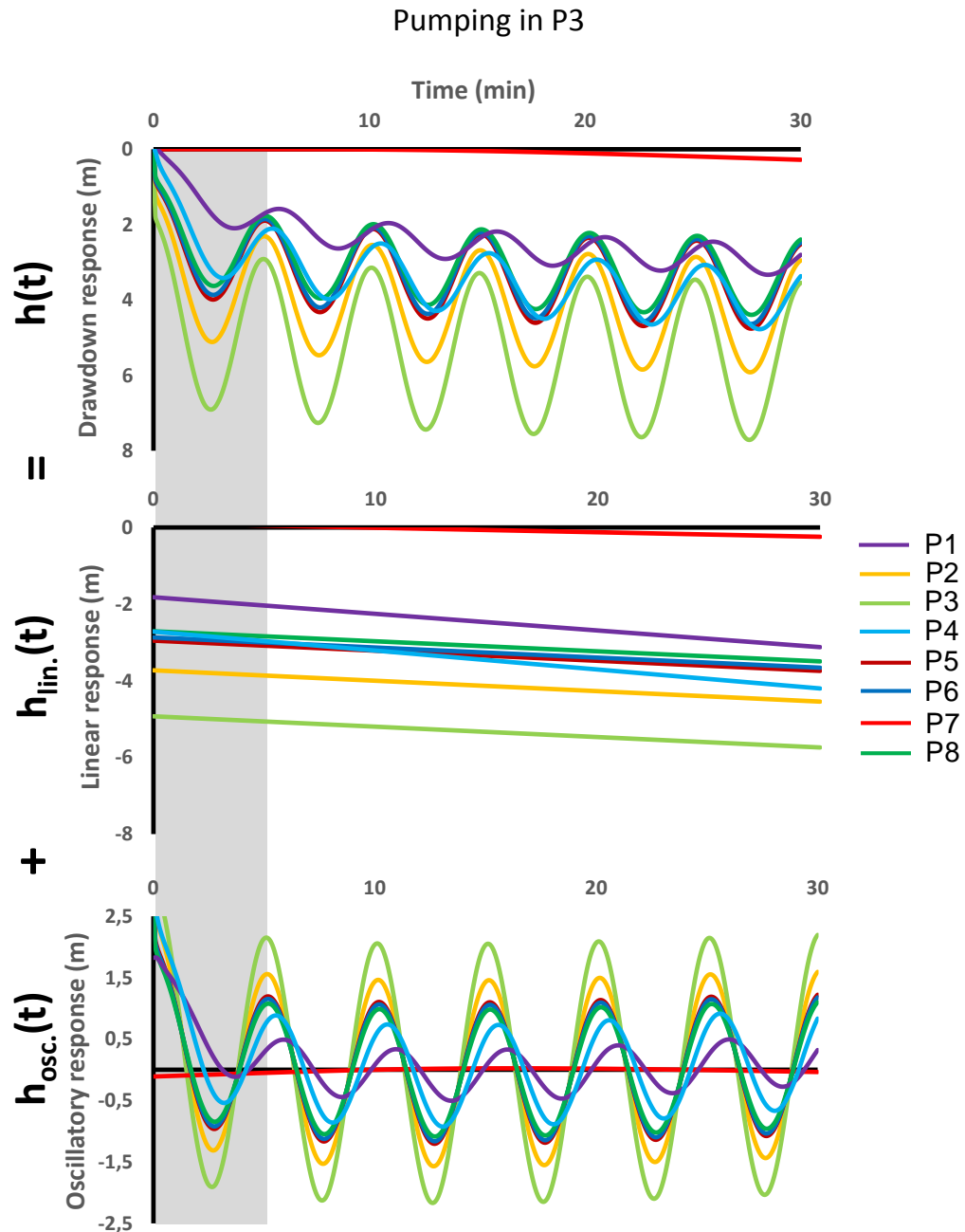
217 Figure 2: Drawdown responses h in each borehole to a harmonic pumping in P3 in a time 218 domain simulation. If the greyed portion of the time series is not considered, these drawdown
