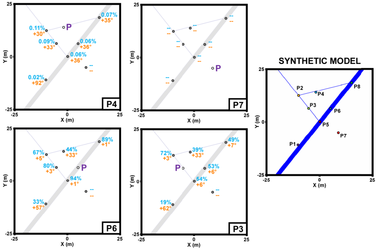
Figure 4: Relative amplitude (% , in blue) and relative phase offset (° , in orange) values in the oscillatory responses in each borehole for different harmonic pumping locations (P4, P7, P6, P3). A dash represents an absence of oscillatory response (< 1 mm). The pumping location is indicated by 'P' and its drawdown oscillatory signal is considered as a 100% amplitude signal with a 0° phase offset.
