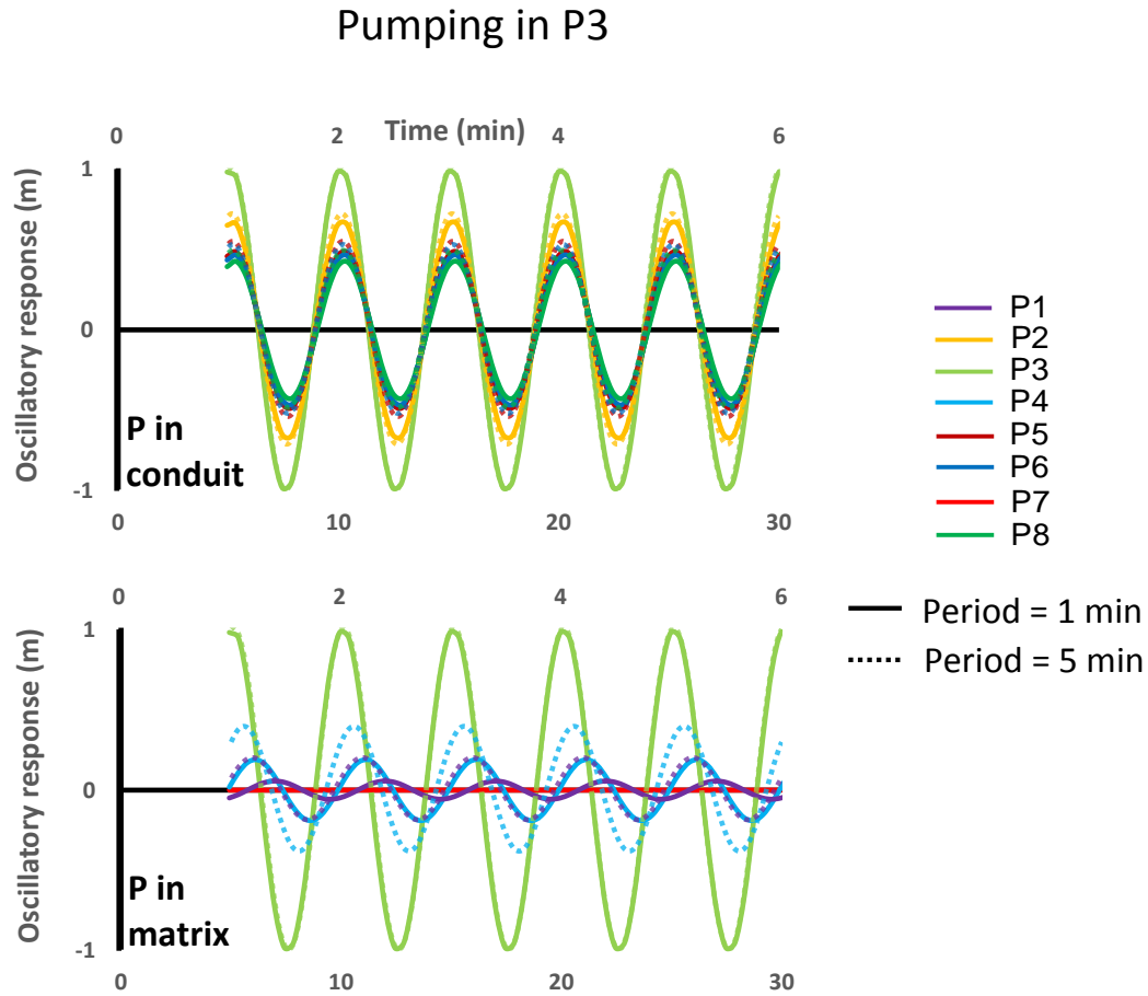
Figure 6: Comparison of the oscillatory relative responses for a harmonic pumping in P3 for a 1min period signal during 6 min (full line) and a 5min period signal during 30 min (dotted line). The measurement boreholes have been separated regarding their location: in a conduit (P2, P5, P6, P8) or in the matrix (P1, P4, P7). The main signal differences appear for the boreholes located in the matrix, near to a conduit (P1, P4) (dual connection).
