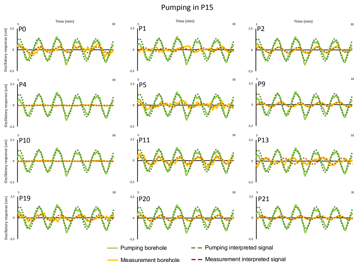
Figure 12: Registered oscillatory responses for each measurement borehole compared to the T=5 min period pumping borehole signal (full lines) and the interpreted signals for an equation form of Eq. 10 with variables amplitude and phase offset values (dotted lines).
