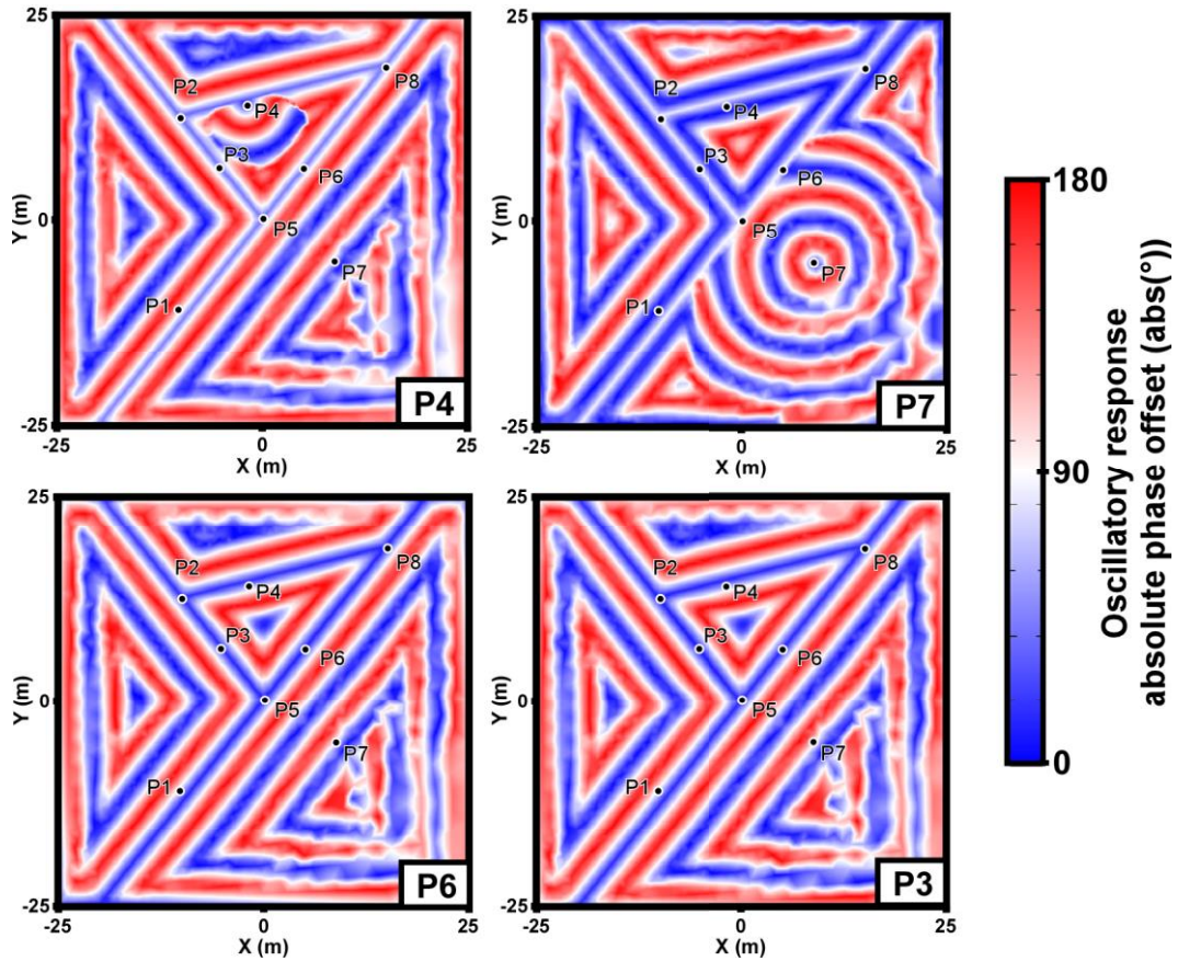
Figure 8: Maps of distribution of the phase offset value in the responses to a harmonic pumping signal with a 5 min period at different locations: in the matrix near a conduit (P4), in the matrix (P7), in a large conduit (P6), in a thin conduit (P3).
