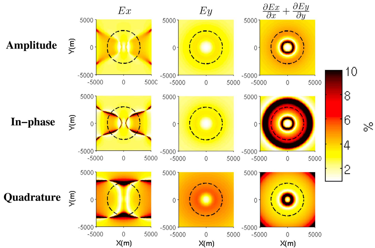
Figure 4. Relative variations (amplitude, in-phase, and quadrature components) for a deep horizontal electric dipole (100 m, 10 A, 1 Hz) between states 1 and 3 of the reservoir (dashed line indicates circle of 3 km radius).
