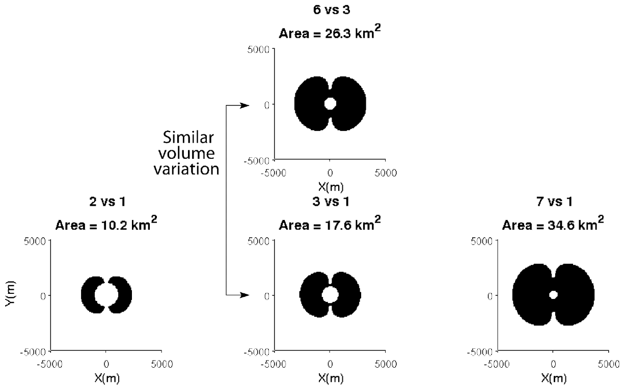
Figure 10. Measurable zone of the Ex component for a deep vertical electric dipole (100 m, 10 A). Conditions are as follows: Relative amplitude variations >1\% and absolute amplitude variations >1 nV/m. The variations represented here are with respect to the initial state 1 of the reservoir. The graph showing the step from state 3 to state 6 has been added for the purposes of comparison with the step from state 1 to state 3, which corresponds to a similar volume of fluid substitution.
