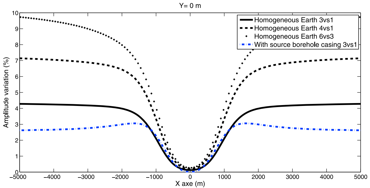
Figure 20. Effect of a steel casing, surrounding the source borehole, on the relative amplitude variation of E_x for a vertical electric dipole (100 m, 10 A, 1 Hz). Profile Y = 0 m. Between states 1 and 3 of the reservoir.
