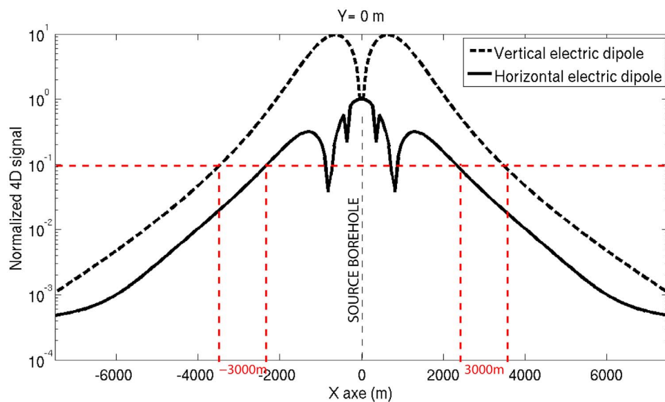
Figure 3. Normalized 4-D signal of the Ex component, between the reservoir's states 1 and 3. Buried vertical or horizontal electric dipole at 1 Hz (100 m, 10 A). Profile Y = 0 m.
