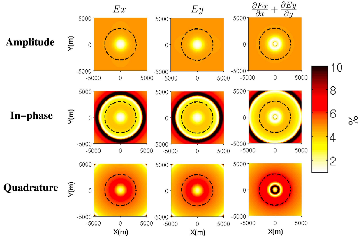
Figure 9. Relative variations (amplitude, in-phase, and quadrature components) for a deep vertical electric dipole (100 m, 10 A, 1 Hz), between states 1 and 3 of the reservoir (dashed line: circle of 3 km radius).
