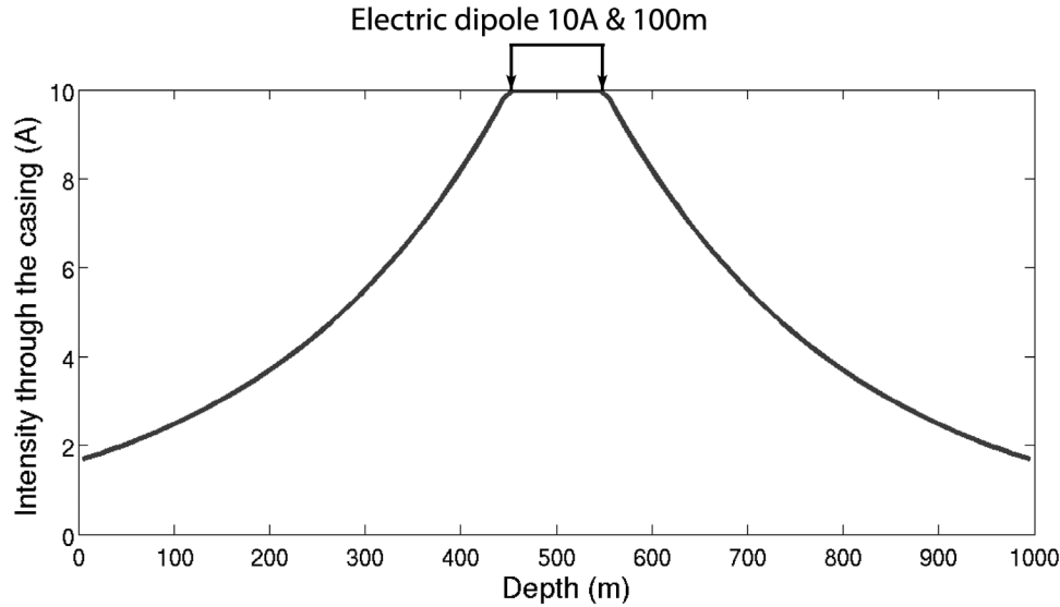
Figure 19. Electric current distribution inside a steel casing ( \sigma = 10^6 S/m) surrounding the source borehole (from equation (11)).
