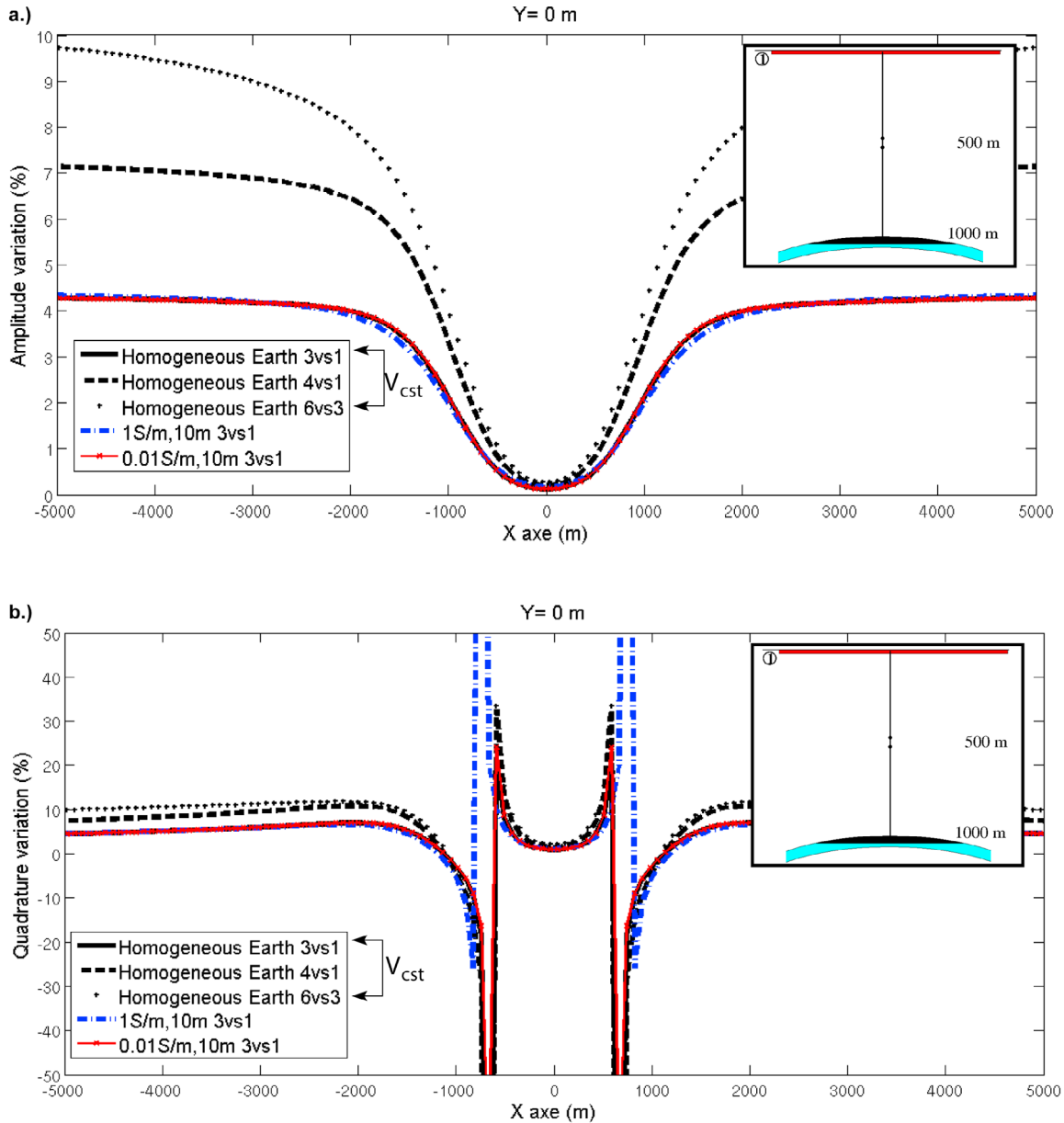
Figure 16. Effect of a near-surface thin layer on the relative amplitude variation for a vertical electric dipole (100 m, 10 A, 1 Hz). Profile Y = 0 m. (a) On E_x component. (b) On \partial E_z / \partial z computed from E_x and E_y (equation (10)).
