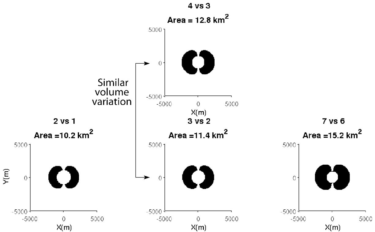
Figure 11. Measurable zone of the E_x component for a deep vertical electric dipole. Conditions are as follows: Relative amplitude variations >1\% and absolute amplitude variations >1 nV/m. The variations represented here are with respect to the previous state (i-1) of the reservoir. The graph showing the step from state 3 to state 4 has been added for the purposes of comparison with the step from state 2 to state 3, which corresponds to a similar volume of fluid substitution.
