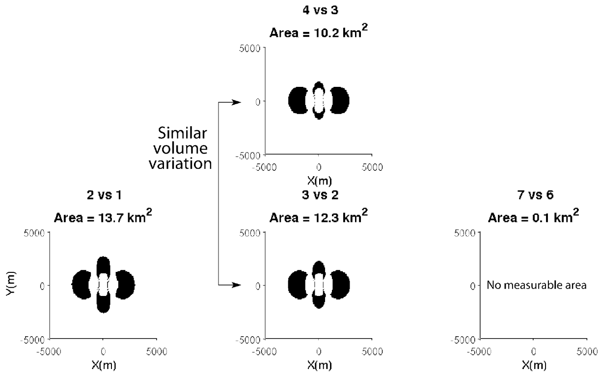
Figure 6. Measurable zone of the E_x component, for a deep horizontal electric dipole (100 m, 10 A, 1 Hz). Conditions are as follows: Relative amplitude variations >1\% and absolute amplitude variations >1 nV/m. The variations represented here are with respect to the previous state ( i-1 ) of the reservoir. The graph showing the step from state 3 to state 4 has been added for the purposes of comparison with the step from state 2 to state 3, which corresponds to a similar volume of fluid substitution.
