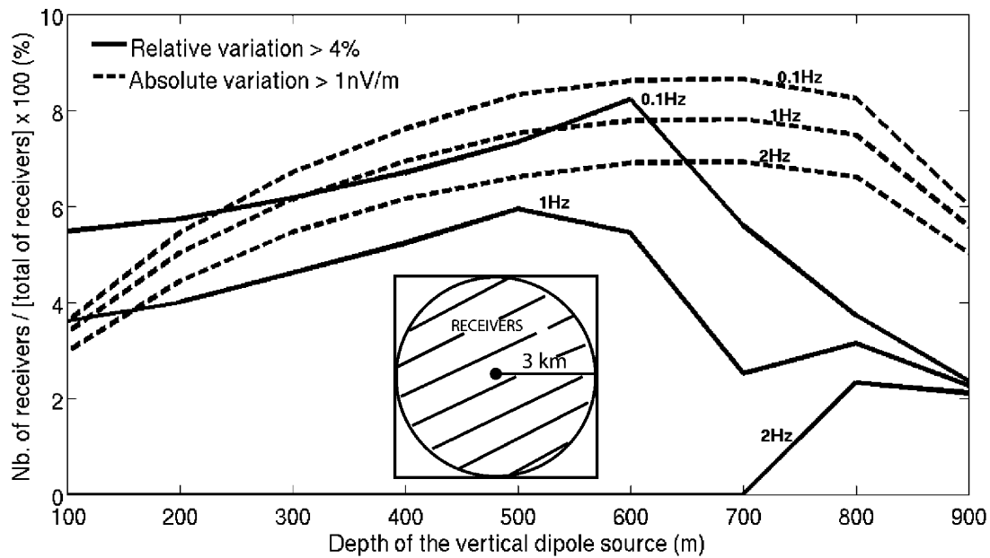
Figure 2. Number of receivers (Ex component) for which the relative variation in amplitude is greater than 4% (solid lines) and for which the 4-D amplitude signal is stronger than 1 nV/m (dashed lines). Time-lapse signal between states 1 and 3 (3vs1, compare Table 1). Variation as a function of the depth of a vertical electric dipole (10 A, 100 m). All of the receivers are arranged on the Earth's surface, within a radius of 3 km centered on the borehole containing the source.
