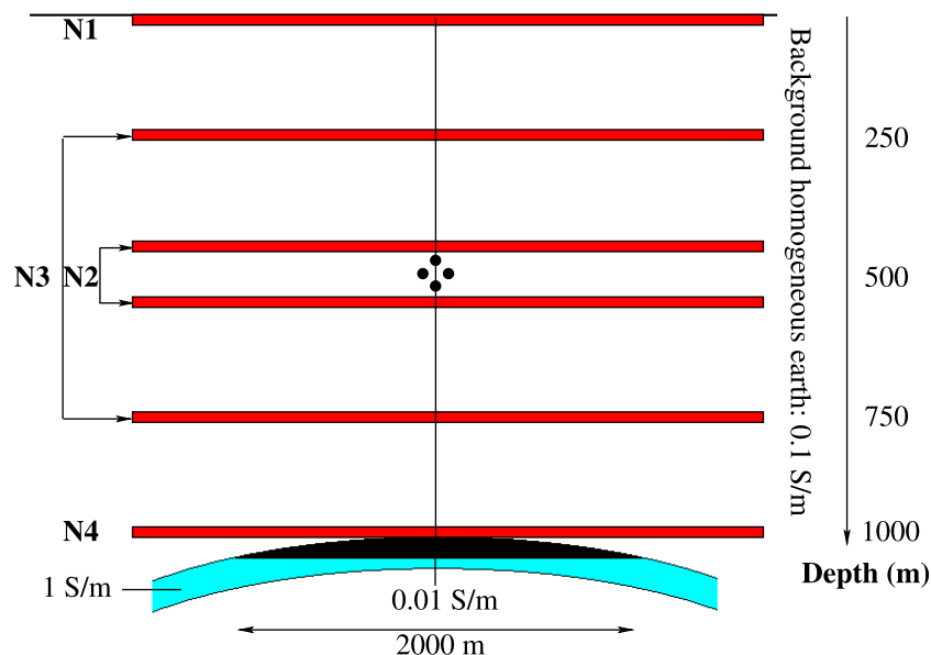
Figure 12. Synthetic case. Lack of knowledge of the background: 10 m conductive thin layer (1 S/m), or resistive thin layer (0.01 S/m) missed. N1, near surface; N2, near source; N3, intermediate distance; N4, near reservoir.
