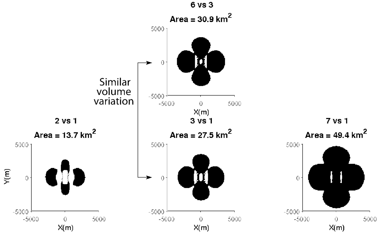
Figure 5. Measurable zone of the E_x component for a deep horizontal electric dipole (100 m, 10 A, 1 Hz). Conditions are as follows: Relative amplitude variations >1\% and absolute amplitude variations >1 nV/m. The variations are based on a comparison with the initial state 1 of the reservoir. The step from state 3 to state 6 (indicated by 6vs3) has been added for comparison with the step from state 1 to state 3, which corresponds to a similar volume of fluid substitution.
