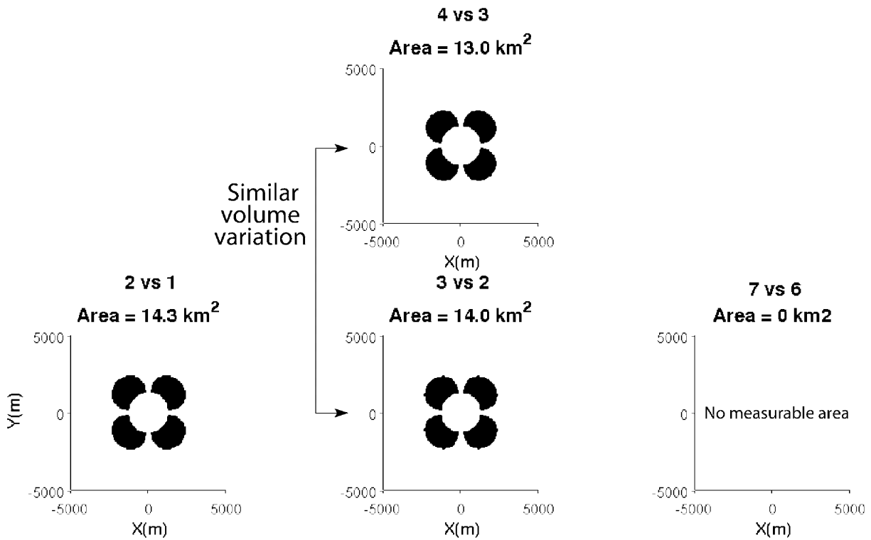
Figure 8. Measurable zone of the E_y component for a deep horizontal electric dipole (100 m, 10 A, 1 Hz). Conditions are as follows: Relative amplitude variations >1\% and absolute amplitude variations >1 nV/m. The variations represented here are with respect to the previous state (i-1) of the reservoir. The graph showing the step from state 3 to state 4 has been added for the purposes of comparison with the step from state 2 to state 3, which corresponds to a similar volume of fluid substitution.
