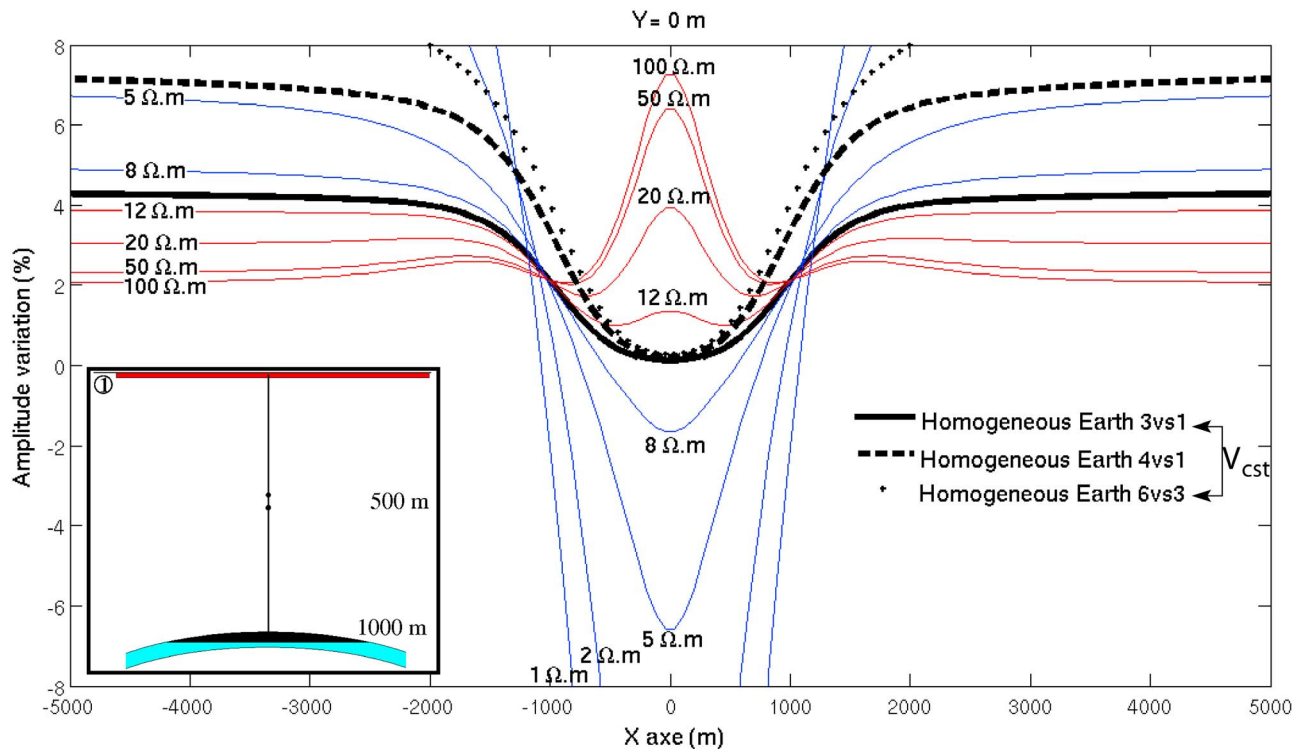
Figure 18. Effect of a change in near-surface conductivity, on the relative amplitude variation of the 4-D signal of the reservoir between states 1 and 3, for different changes in conductivity in the first 10 m (initially at 10 \Omega m to 0.1 S/m). Profile of E_x component at Y = 0 m. Vertical electric dipole (100 m, 10 A, 1 Hz). The conductivity changes range from 0.01 to 1 S/m.
