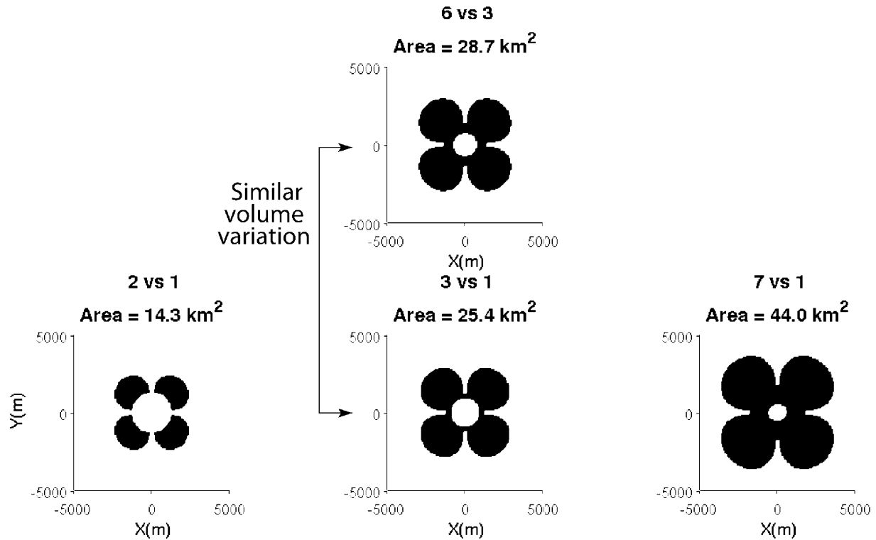
Figure 7. Measurable zone of the E_y component for a deep horizontal electric dipole (100 m, 10 A, 1 Hz). Conditions are as follows: Relative amplitude variations >1\% and absolute amplitude variations >1 nV/m. The variations represented here are with respect to the initial state 1 of the reservoir. The graph showing the step from state 3 to state 6 has been added for the purposes of comparison with the step from state 1 to state 3, which corresponds to a similar volume of fluid substitution.
