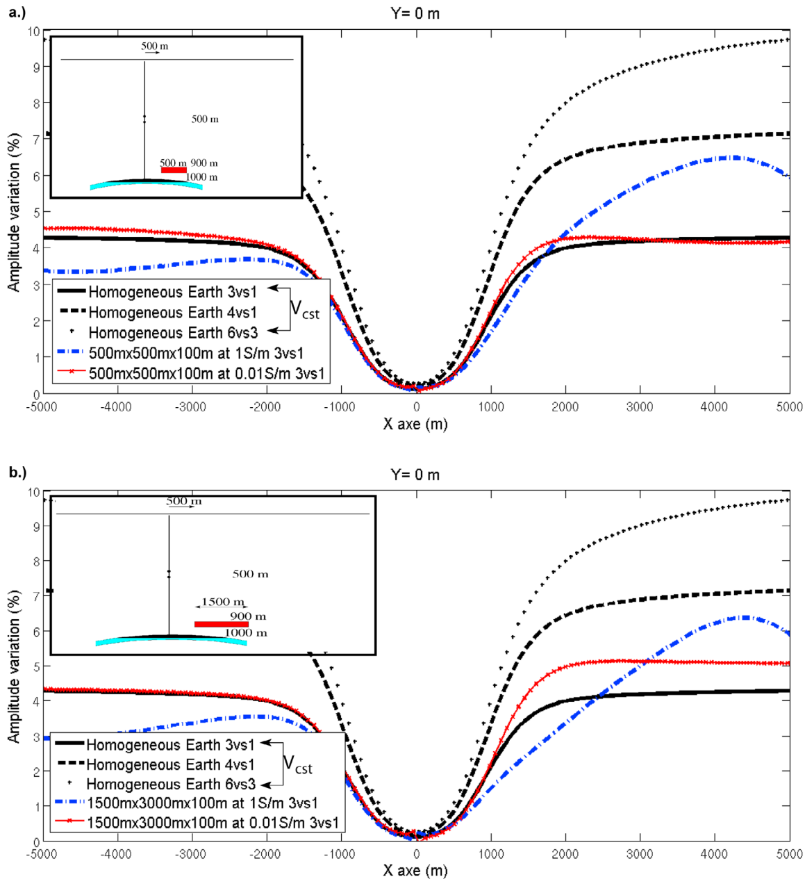
Figure 15. Effect of a near-reservoir 3-D body on the relative amplitude variation of E_x for a vertical electric dipole (100 m, 10 A, 1 Hz). Profile Y = 0 m. (a) Small, 500 m \times 500 m \times 100 m, 3-D body. (b) Large, 1500 m \times 3000 m \times 100 m, 3-D body.
