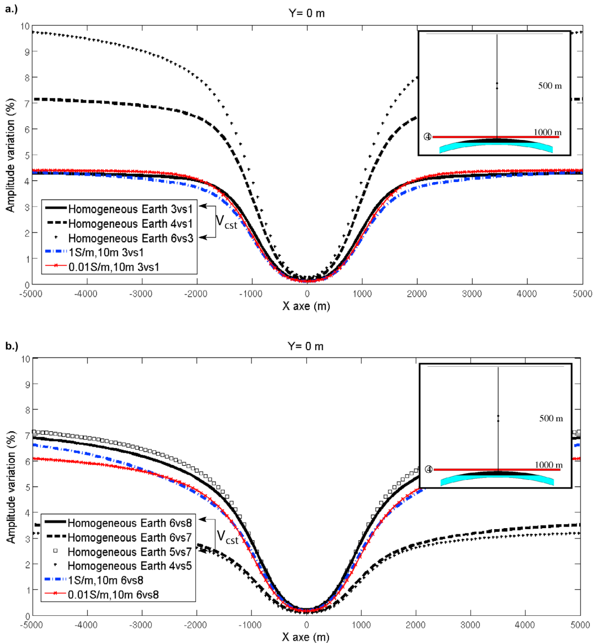
Figure 14. Effect of a near-reservoir thin layer on the relative amplitude variation of E_x , for a vertical electric dipole (100 m, 10 A, 1 Hz). Profile Y = 0 m. (a) Between states 1 and 3 of the reservoir. (b) Between the last states, 6 and 8, of the reservoir.
