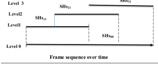
Fig. 4. A 3-level representation of Temporal construction of the SHs, SH_{l,j} is the j^{\text{th}} Spherical harmonics in the l^{\text{th}} level of the hierarchy
