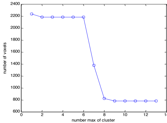
Figure 7. (a) Variation in the number of voxels by number max of clusters k .
